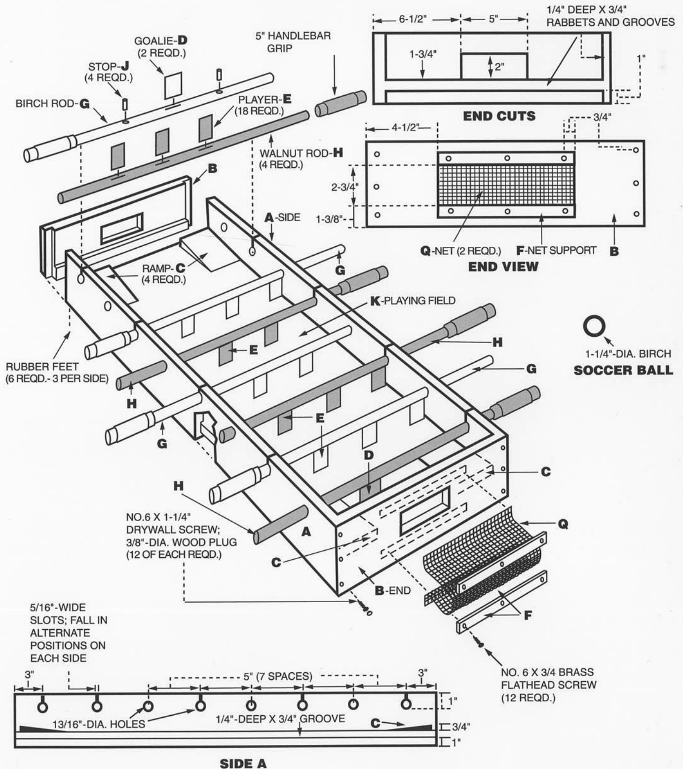
FIG A. TABLETOP SOCCER ASSEMBLY
